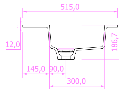
C-C ( 1:10 )
