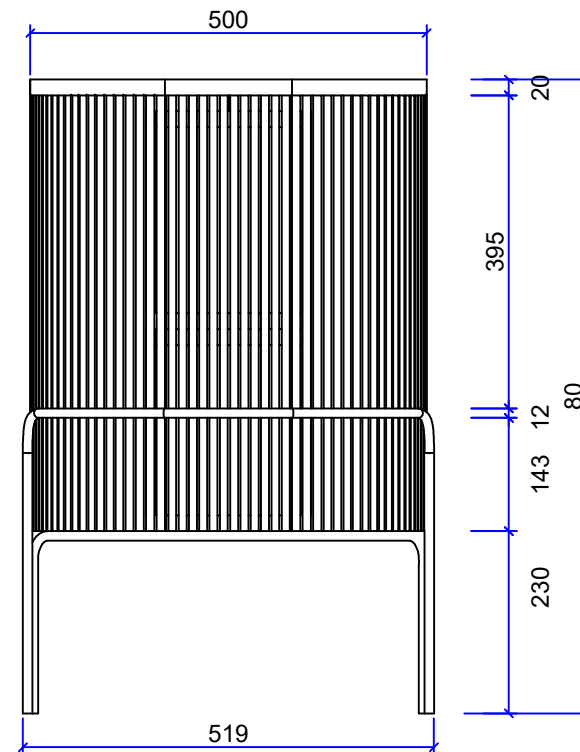
SIDE VIEW SCALE 1:10
