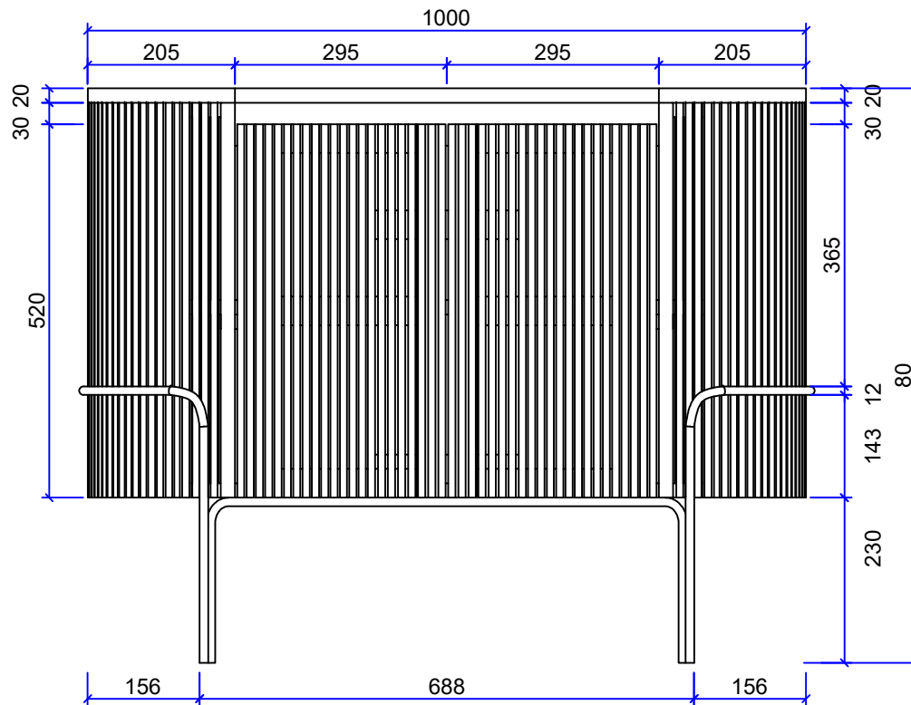
FRONT VIEW SCALE 1:10
