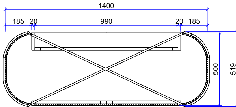
BOTTOM VIEW SCALE 1:10
