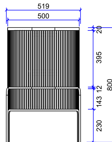
SIDE VIEW SCALE 1:10
